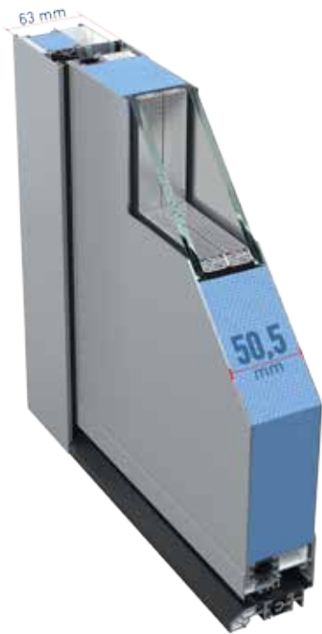
TLS50 FLAT frame
