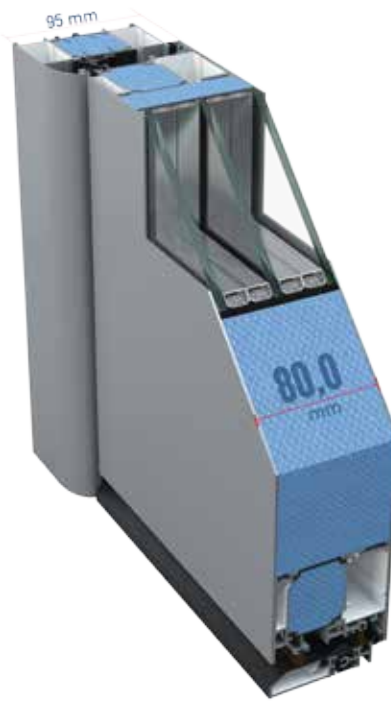
TLS90 CURVED frame
